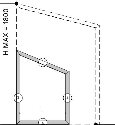
L MAX = 700
