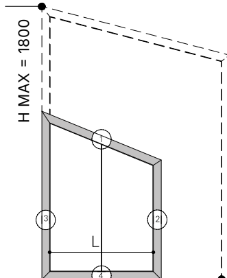
L MAX = 1400 (700+700)
